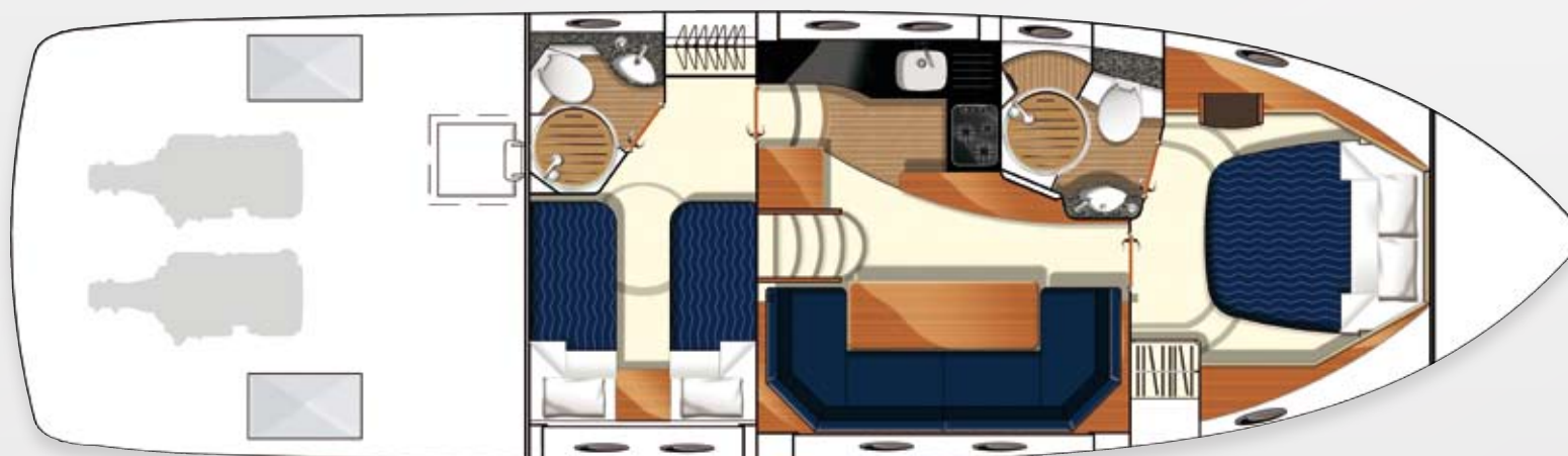
Lower accommodation layout
